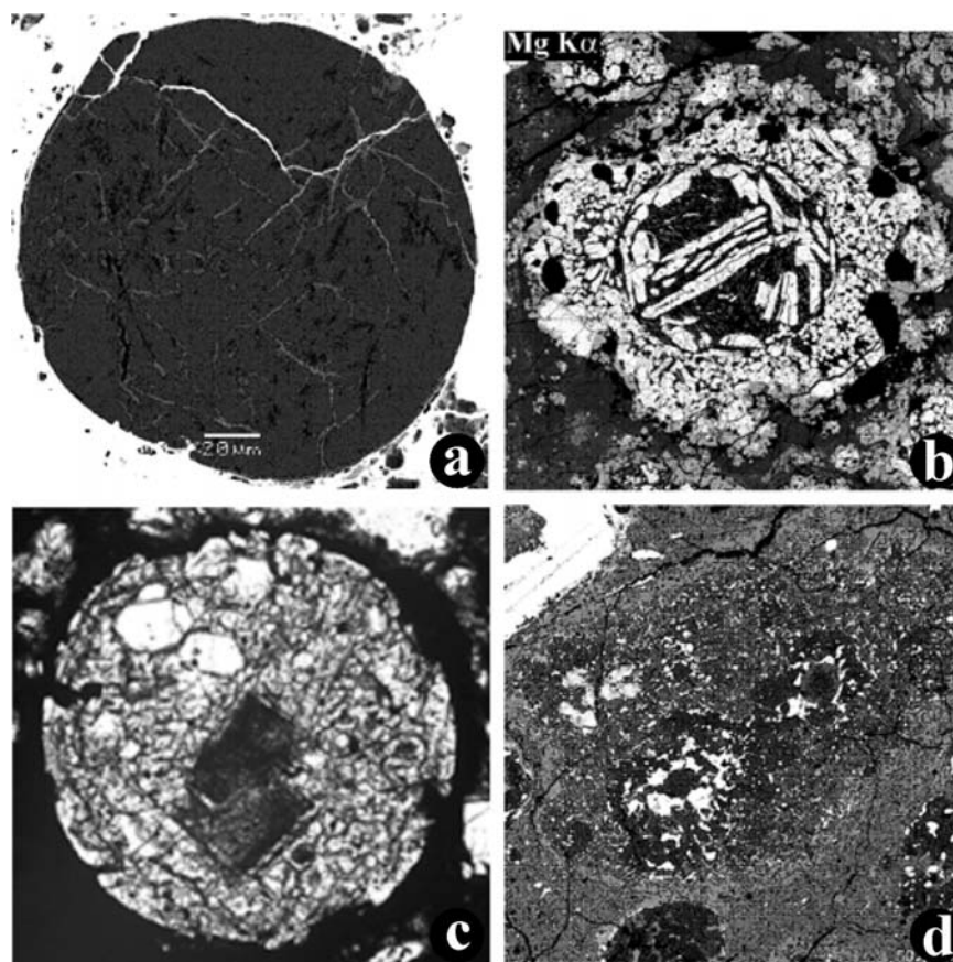
Figure 2. (a) Cryptocrystalline chondrule from the CB chondrite Hamradah al Hamra 237, BSE. (b) 500- \mu\text{m} thick igneous rim on 1 mm BO/PO chondrule in the CV chondrite Efremovka, Mg X-ray image. (c) 750- \mu\text{m} diameter Type IAB chondrule in Chainpur with dusty olivine relict grains, PPL. (d) Chondrule in the CR chondrite Renazzo 1.5 mm long consisting of an aggregate of coarser grained and finer grained domains, BSE, olivine black, metal white. PPL = ordinary light, BSE = back-scattered electrons. (a) and (b) courtesy of A. Krot.
