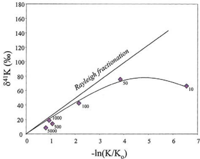
Figure 14. Fraction of K retained and isotopic composition for charges heated at a P_{\text{H}_2} of 1.3 \times 10^{-7} bars in covered capsules, as a function of cooling rate between 5000^\circ\text{C/hr} and 10^\circ\text{C/hr} . K isotopic fractionation is partially suppressed for low cooling rates because of back reaction with the ambient gas (Cohen et al. 2004).
