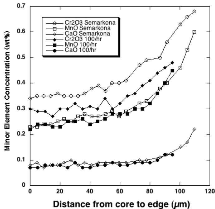
Figure 9. Minor element zoning profiles for olivine in a IIA charge cooled at 100 °/hr and in a chondrule (after Jones & Lofgren 1993; Connolly et al. 2005).
